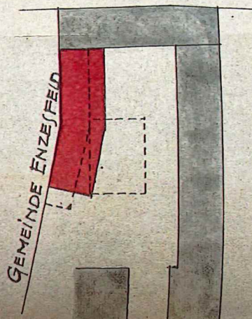
SITUATION 1:500
